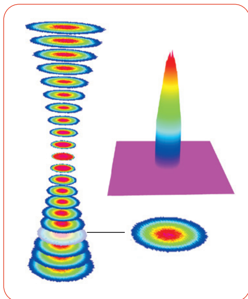
Display of a caustic measurement of a multi mode laser by the LaserDiagnosticsSoftware.
