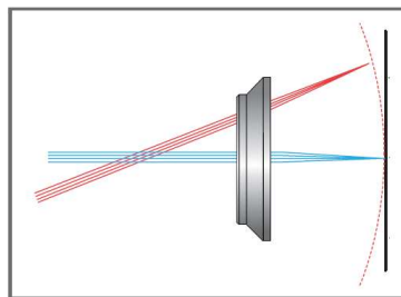
(a)Singlet
