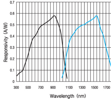
S/G 2-COLOR PHOTODETECTOR Typical Spectral Response - 22°C
