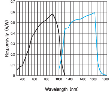
S/IGA 2-COLOR PHOTODETECTOR Typical Spectral Response - 22°C
