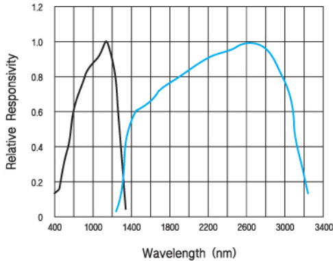
S/PBS 2-COLOR PHOTODETECTOR Typical Spectral Response - 22°C
