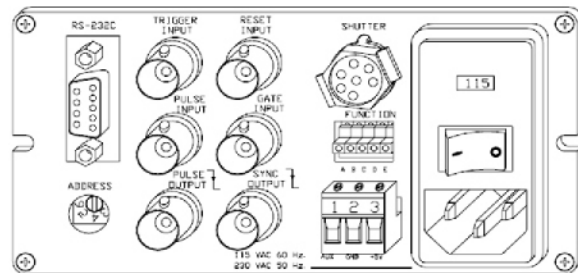
VMM-T1 Rear Panel
