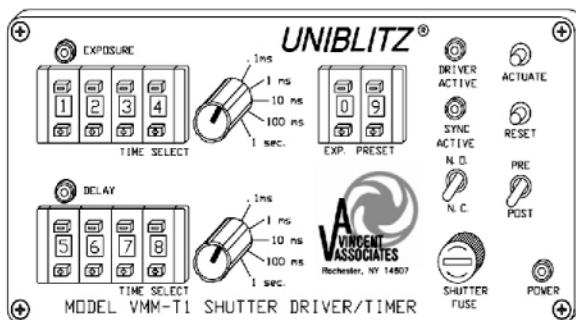
VMM-T1 Front Panel
